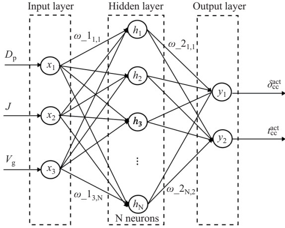
Fig. 13. ANN method for estimating \delta_{cc}^{\text{act}} and t_{cc}^{\text{act}} .
