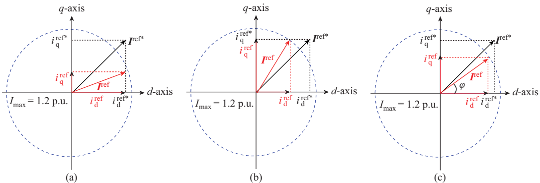
Fig. 3. Priority-based current-limiting approach. (a) d -axis priority. (b) q -axis priority. (c) Phase angle priority.
