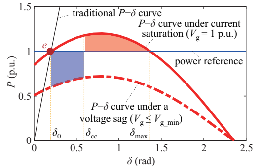
Fig. 9. P - \delta curve under condition 3 ( V_g \leq V_{g\_min} ).
