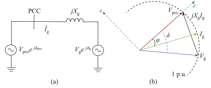
Fig. 2. Phasor diagram of the main circuit. (a) Simplified diagram of the studied power system. (b) Phasor diagram.
