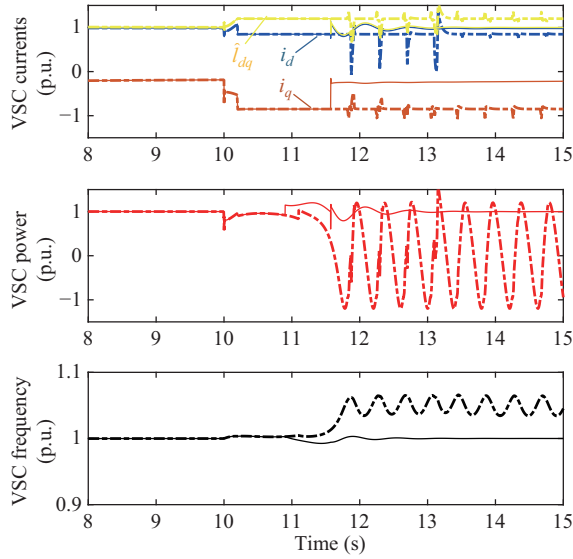
Fig. 19. Results for a 20% voltage sag without the existence of equilibrium points (solid line: t_{cl} = 0.9 s; dashed line: t_{cl} = 1.1 s).
