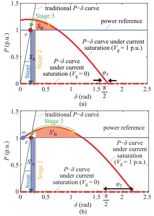
Fig. 4. Trajectories of operating point on P-\delta curve with different \varphi of \mathbf{I}_{dq}^{\text{ref}} . (a) P-\delta curve with a smaller \varphi . (b) P-\delta curve with a larger \varphi .
