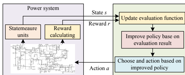
Fig. 1 Framework of reinforcement learning method
